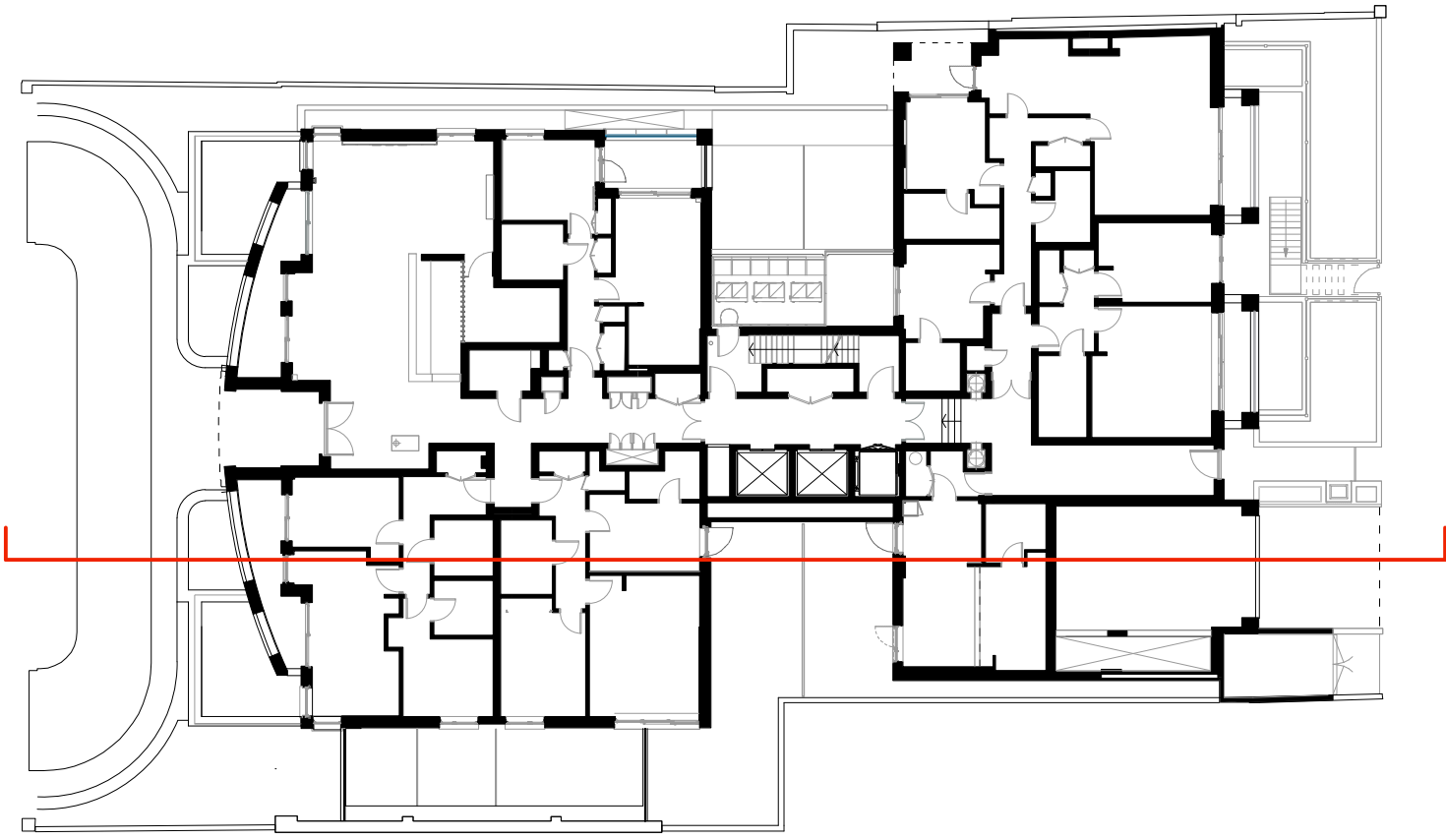
SECTION LOCATION PLAN
