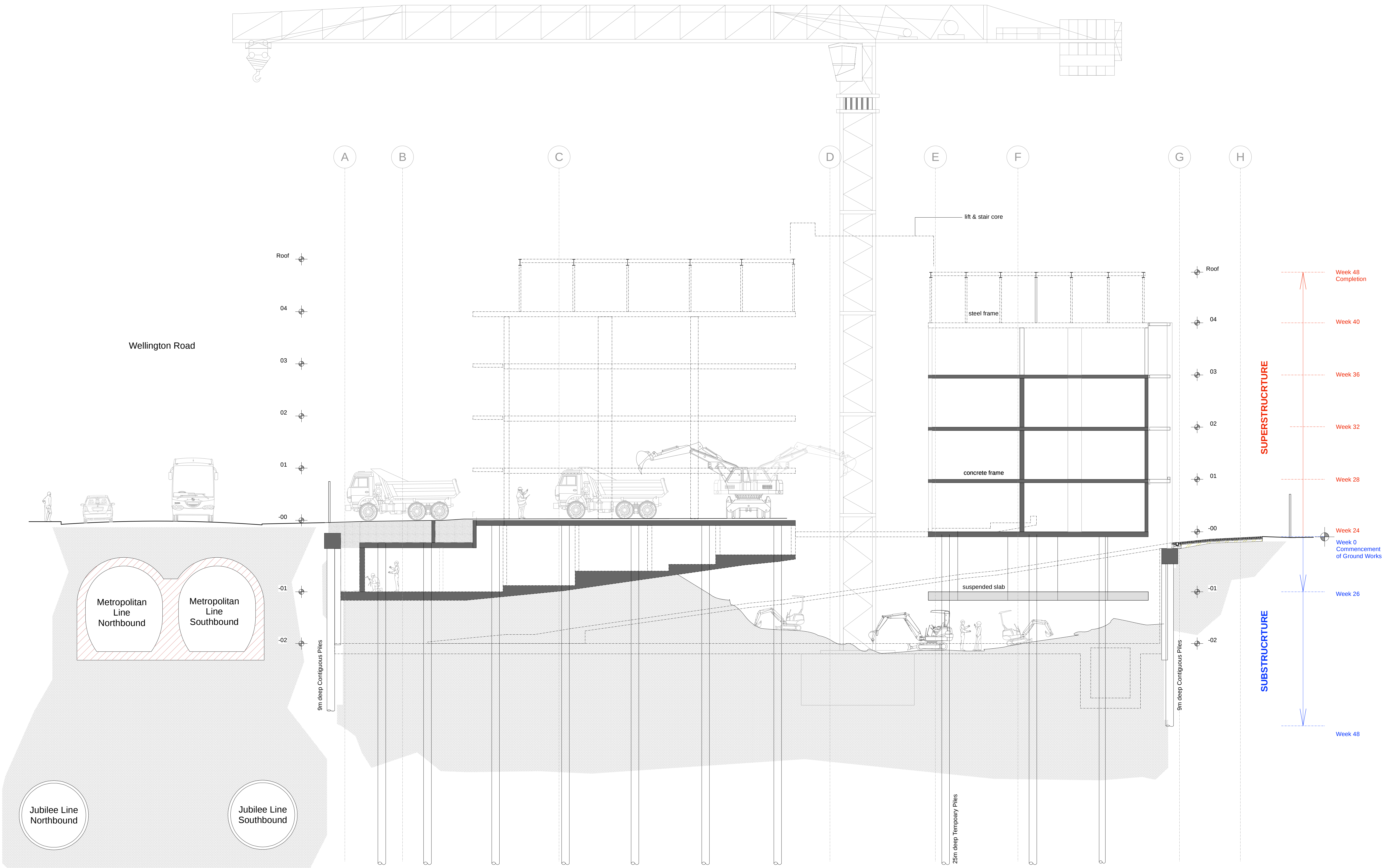
TOP DOWN CONSTRUCTION ILLUSTRATION : 28-32 WELLINGTON ROAD, LONDON NW8
